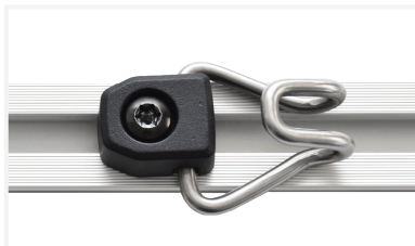
Lashing hook for T-Track M8 Art. No: 39011
